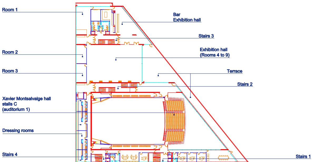
SECOND FLOOR
